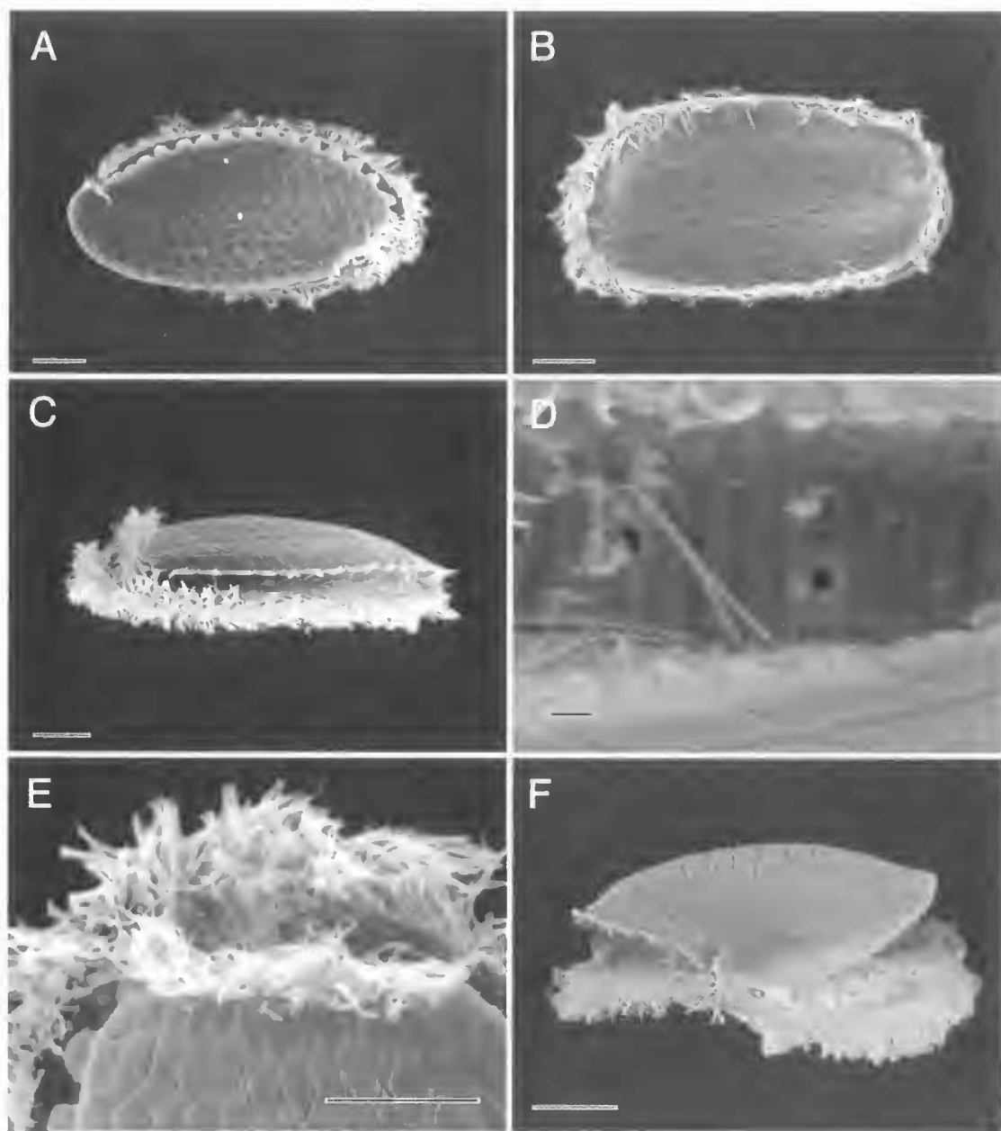
FIG. 3. Scanning electron micrographs of Macropodinium moihi Dehority, 1996. A. right view, scale bar = 10 \mu m. B. left view, scale bar = 10 \mu m. C. dorsal view, scale bar = 10 \mu m. D. contractile vacuole pores in ventral DVG, scale bar = 1 \mu m. E. anterior right view, scale bar = 10 \mu m. F. cytoproct, scale bar = 10 \mu m.
